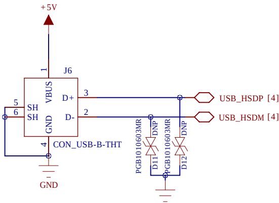
HS USB Device @AP7000
