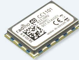
radino40 CC1101 433 MHz · Model 901.614A001 · fully shielded, EMC-compliant
