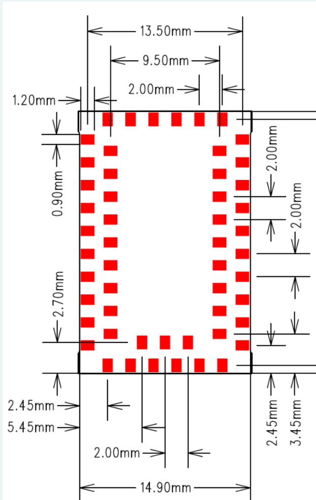
Recommended Land Pattern
