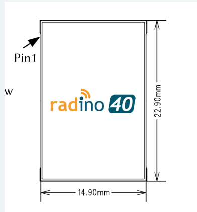
Top view — outline dimensions
