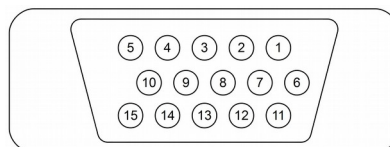
Pinout DE-15 Connectors
